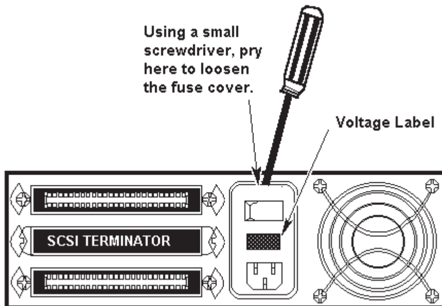
ILLUSTRATION 2-1 REMOVING AC FUSE COVER
